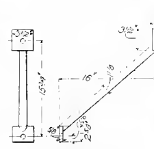
Figs. 4893-94. PEDESTAL-BRACE.
